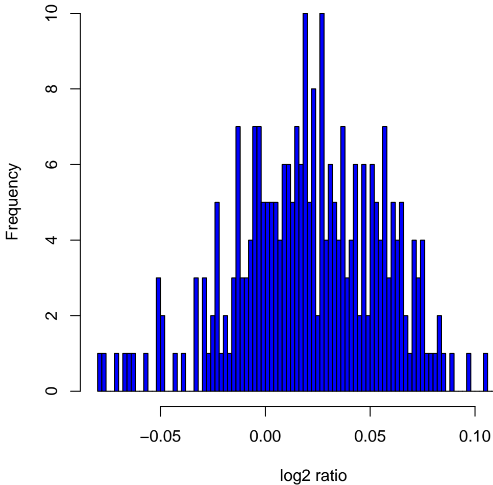
Histogram of log 2 ratios in 270 HapMap samples at clone Chr4tp-9C10
