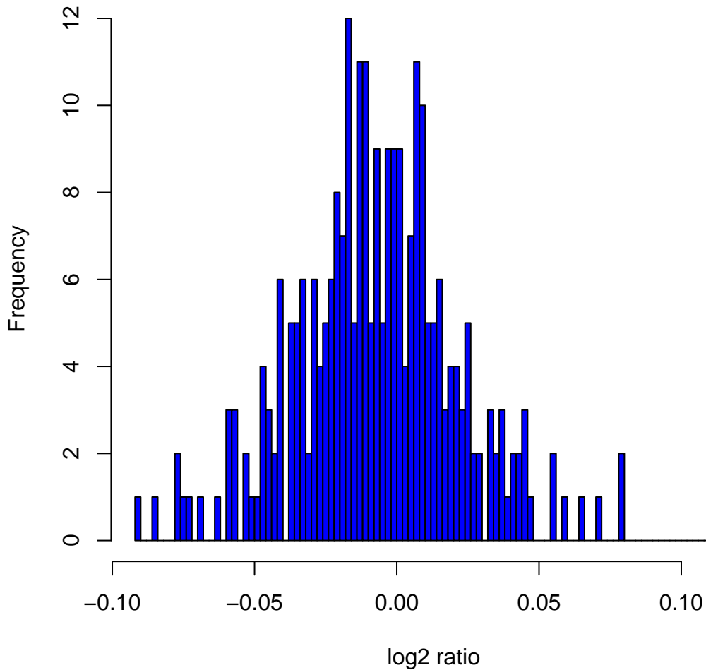
Histogram of log2ratios in 270 HapMap samples at clone Chr4tp-9E3
