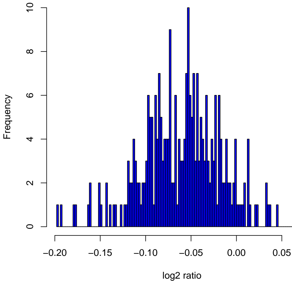
Histogram of \log_2 ratios in 270 HapMap samples at clone Chr4tp-9E8
