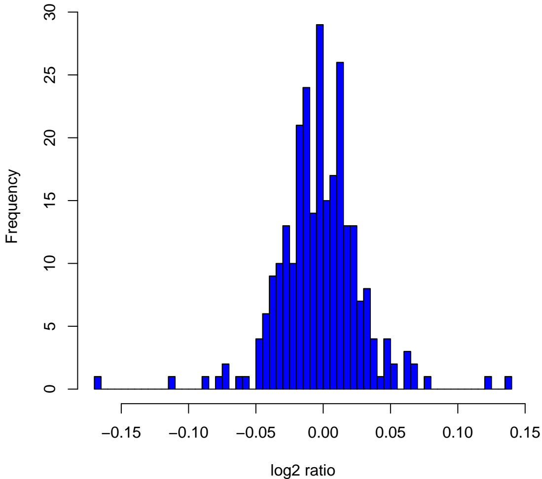
Histogram of log2ratios in 270 HapMap samples at clone Chr4tp-9F12
