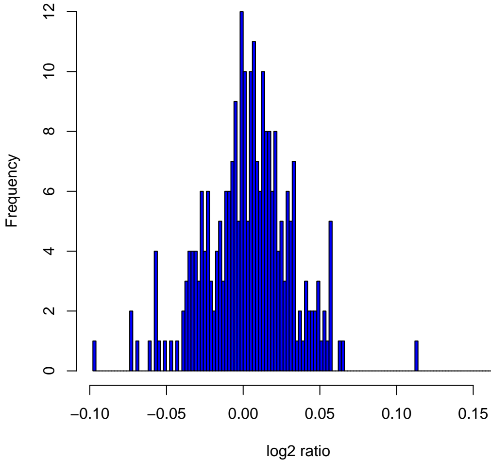
Histogram of log 2 ratios in 270 HapMap samples at clone Chr4tp-9F5
