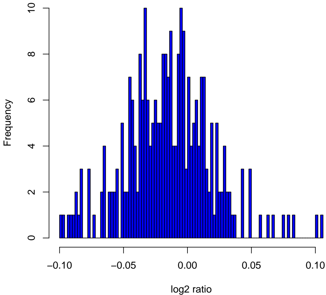
Histogram of log2ratios in 270 HapMap samples at clone Chr4tp-9H7
