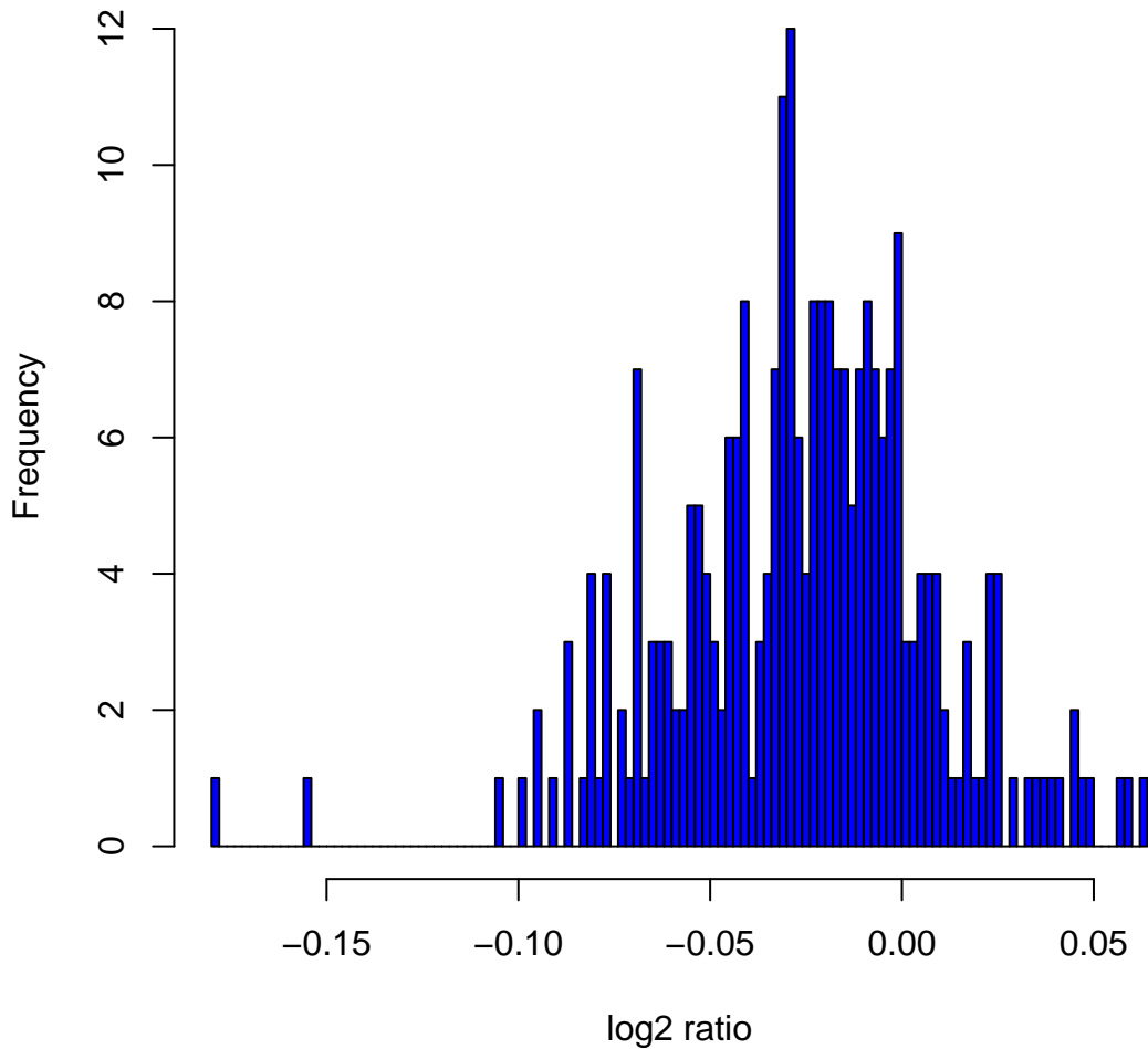
Histogram of log 2 ratios in 270 HapMap samples at clone Chr4tp-9H9
