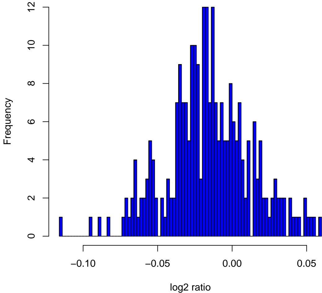
Histogram of log2ratios in 270 HapMap samples at clone Chr5tp-10B11
