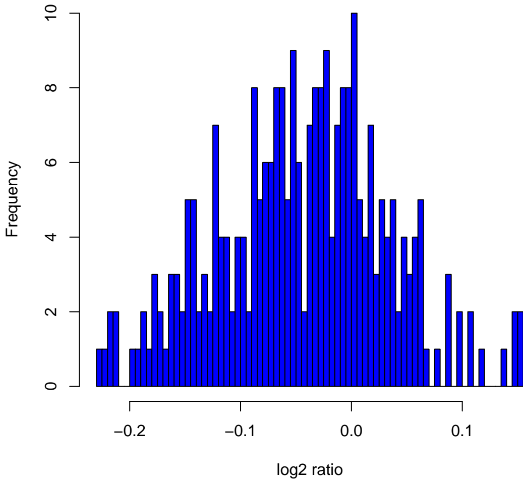
Histogram of log 2 ratios in 270 HapMap samples at clone Chr5tp-10E1
