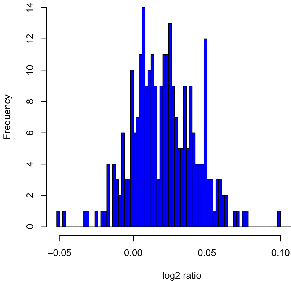
Histogram of \log_2 ratios in 270 HapMap samples at clone Chr5tp-10G6
