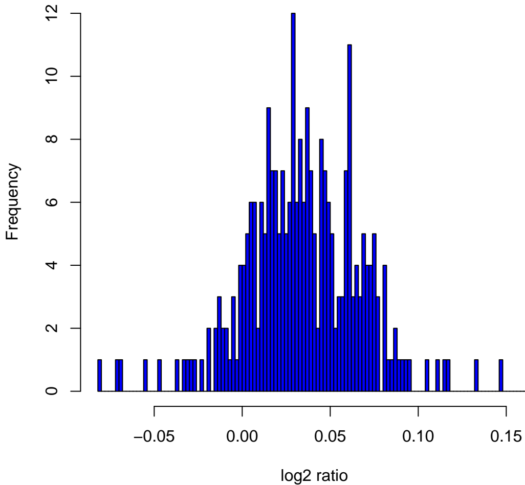
Histogram of log 2 ratios in 270 HapMap samples at clone Chr5tp-11E3
