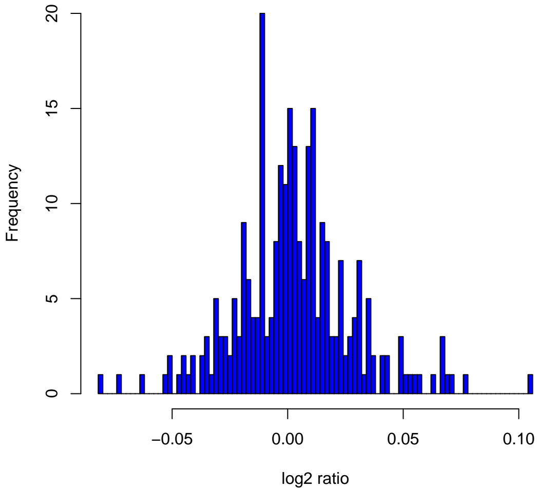
Histogram of log2ratios in 270 HapMap samples at clone Chr5tp-12B12
