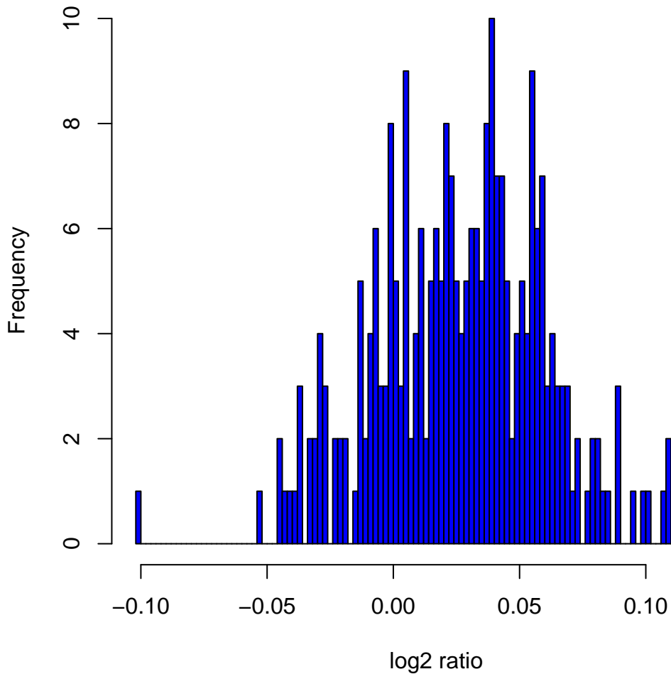
Histogram of \log_2 ratios in 270 HapMap samples at clone Chr5tp-13B7
