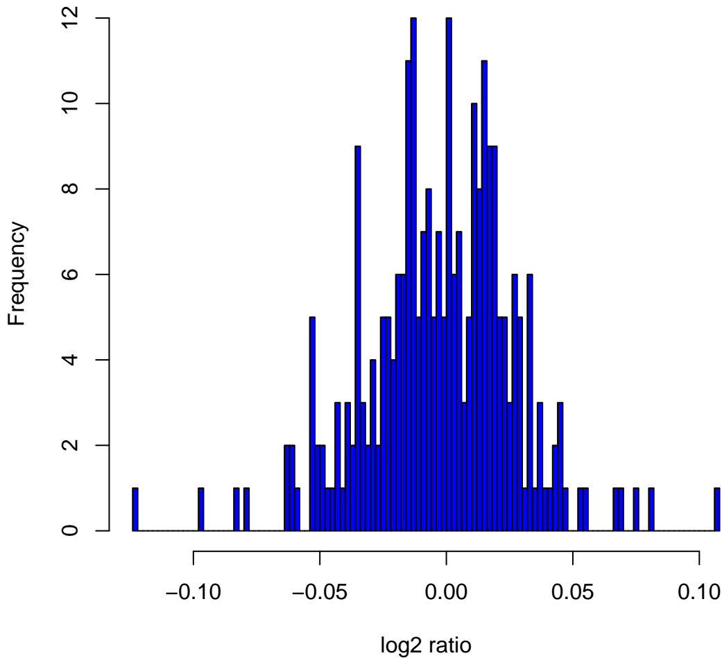
Histogram of log 2 ratios in 270 HapMap samples at clone Chr5tp-13C6
