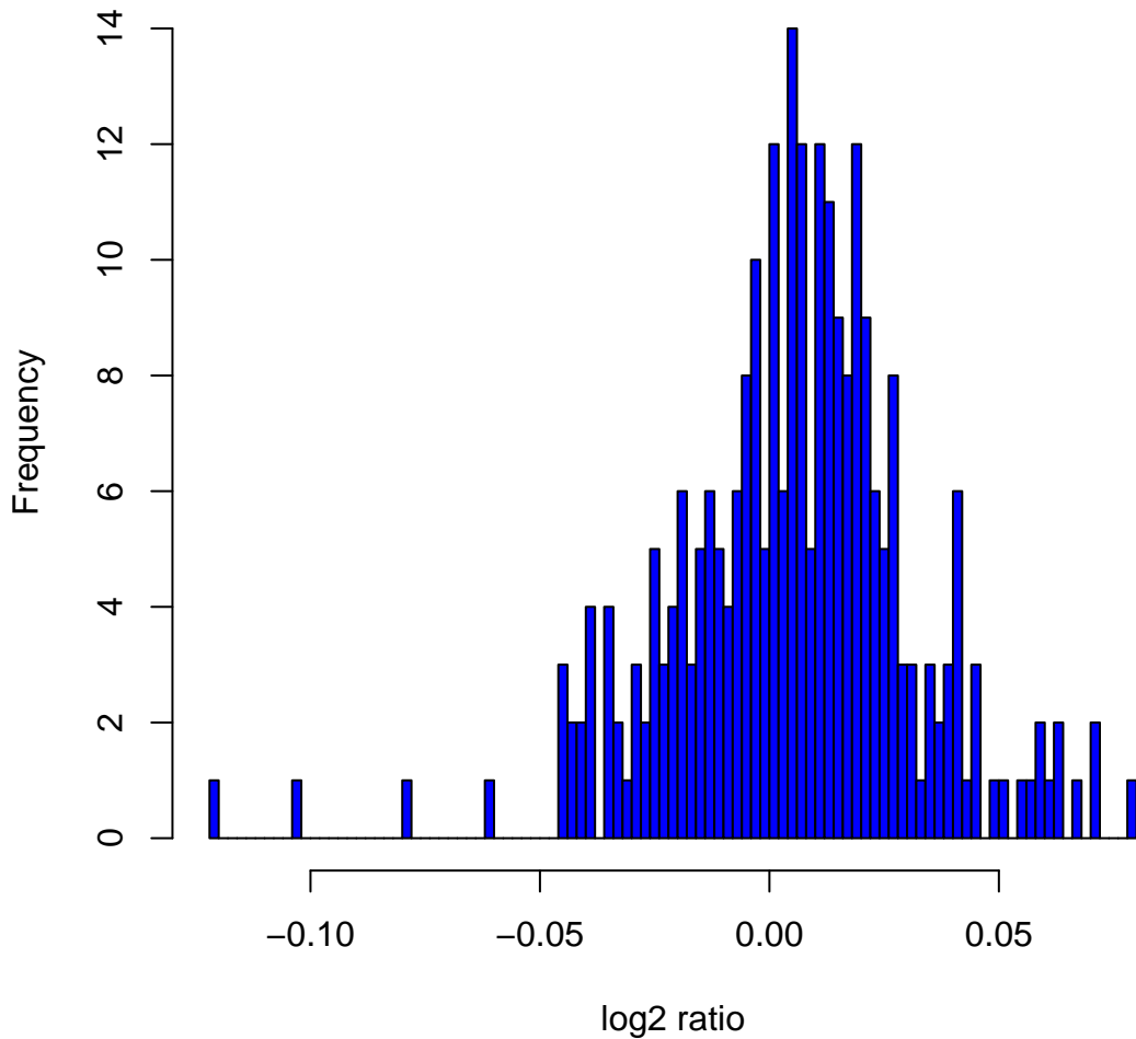
Histogram of log2ratios in 270 HapMap samples at clone Chr5tp-13D12
