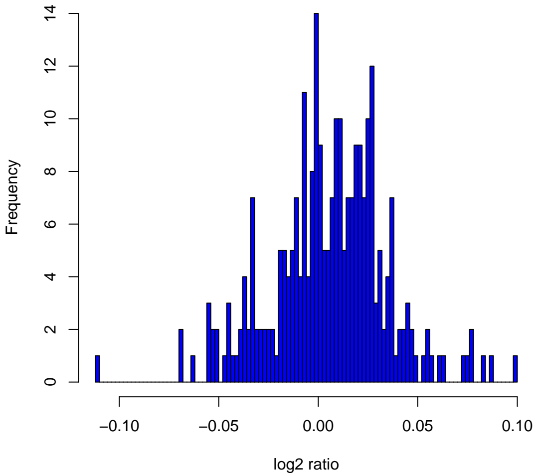
Histogram of log 2 ratios in 270 HapMap samples at clone Chr5tp-15C3
