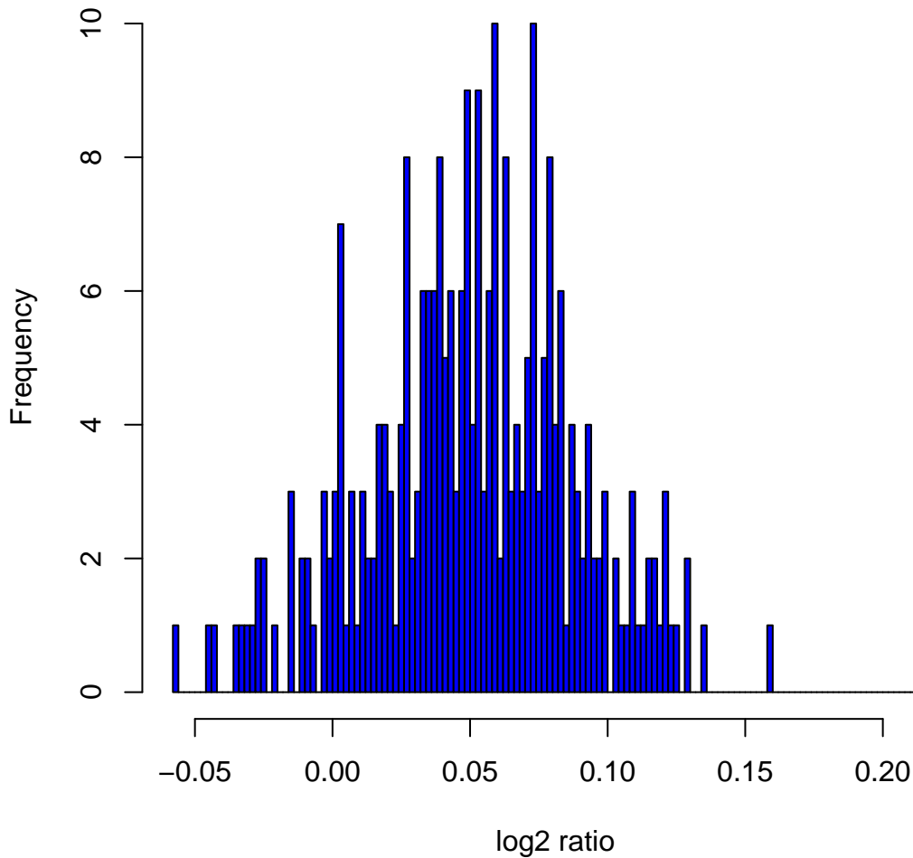
Histogram of log2ratios in 270 HapMap samples at clone Chr5tp-15D11
