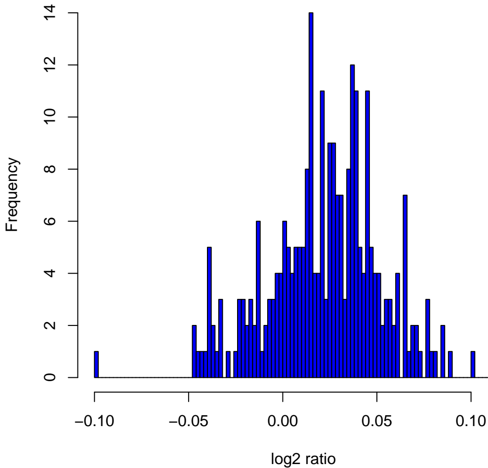
Histogram of \log_2 ratios in 270 HapMap samples at clone Chr5tp-15E1
