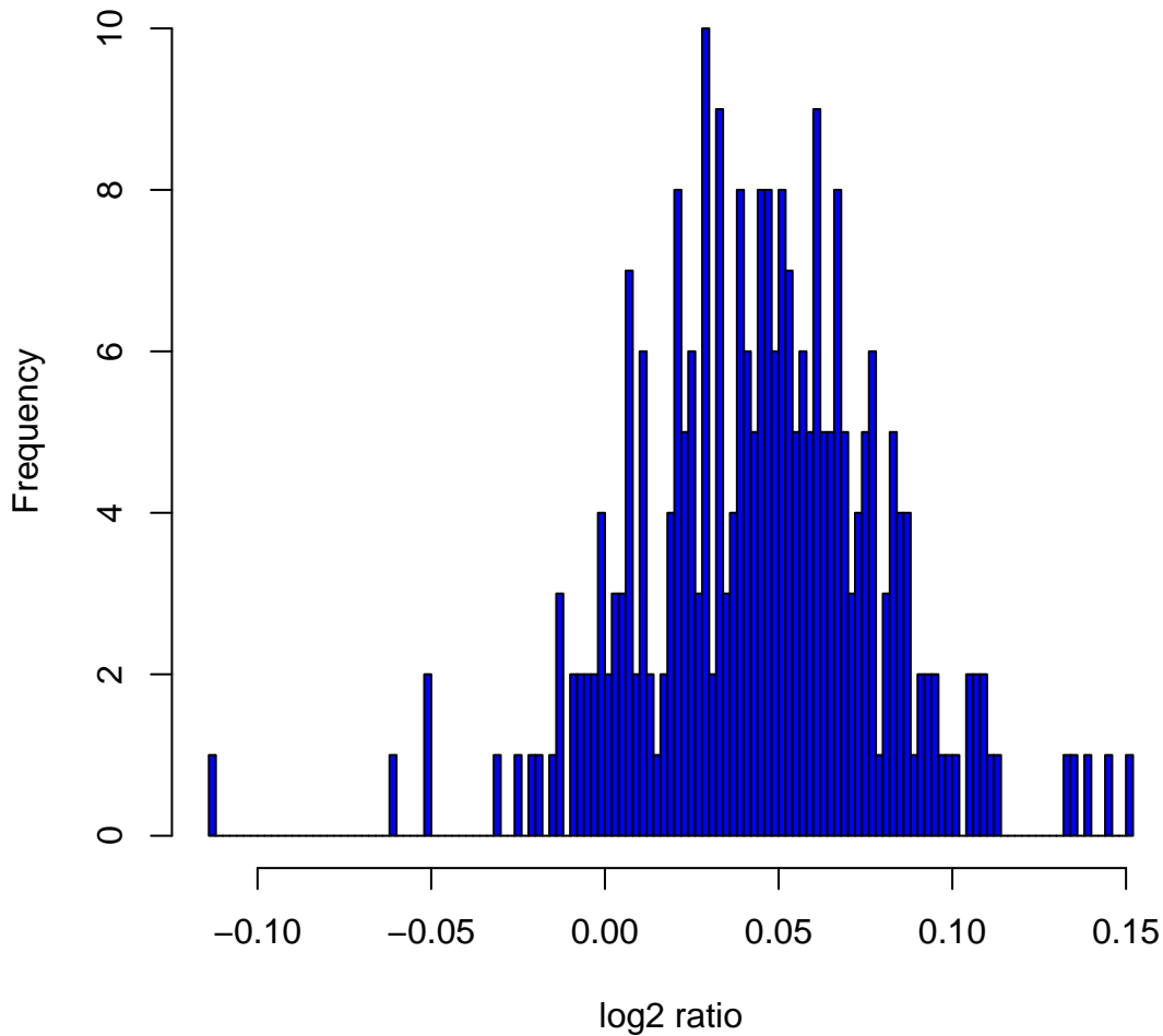
Histogram of log2ratios in 270 HapMap samples at clone Chr5tp-15H12
