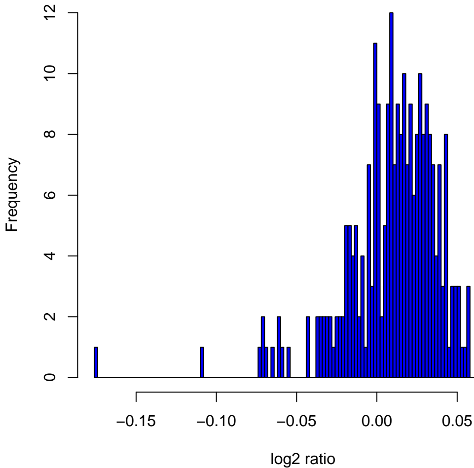
Histogram of log2ratios in 270 HapMap samples at clone Chr5tp-16B4
