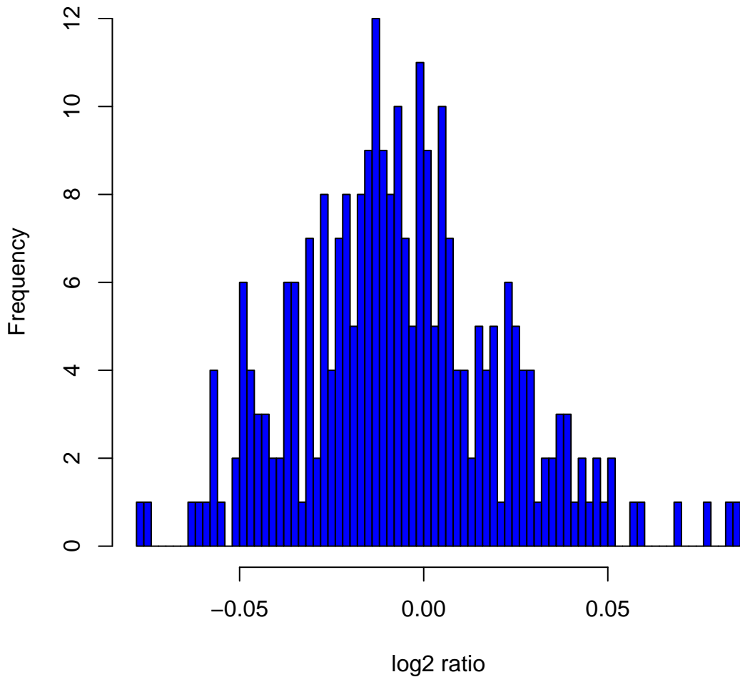
Histogram of log2ratios in 270 HapMap samples at clone Chr5tp-16D12
