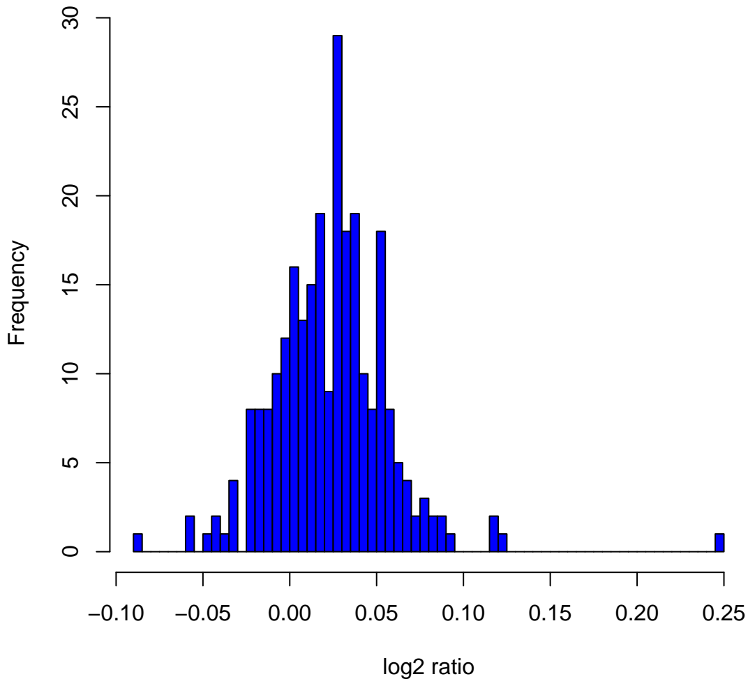
Histogram of \log_2 ratios in 270 HapMap samples at clone Chr5tp-16D2
