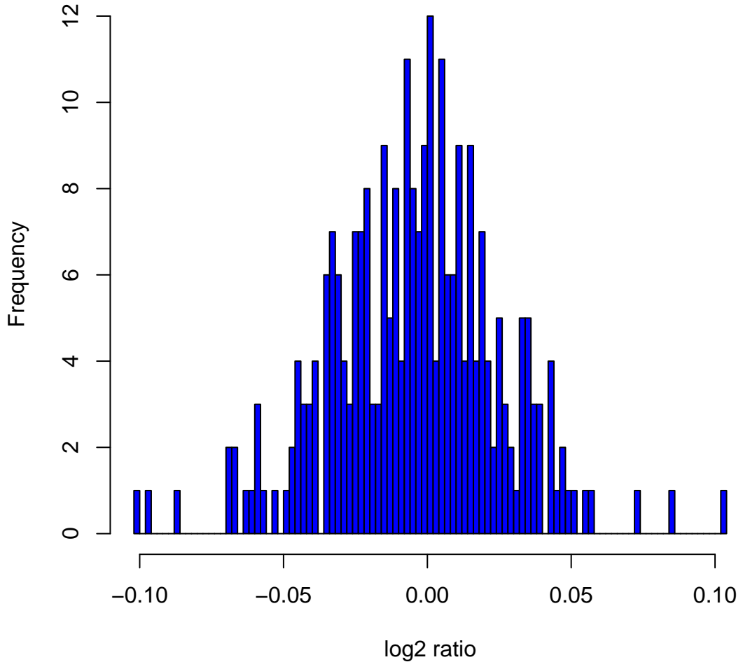
Histogram of \log_2 ratios in 270 HapMap samples at clone Chr5tp-16D4
