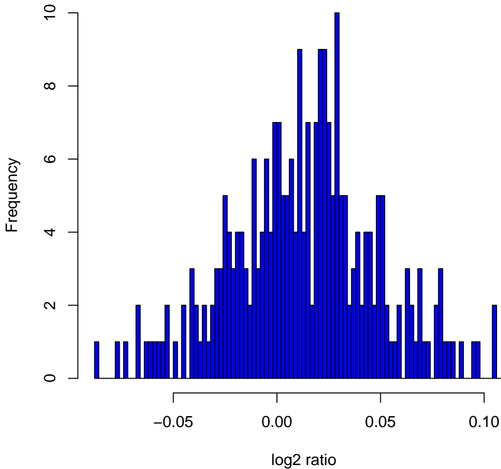
Histogram of \log_2 ratios in 270 HapMap samples at clone Chr5tp-16D7
