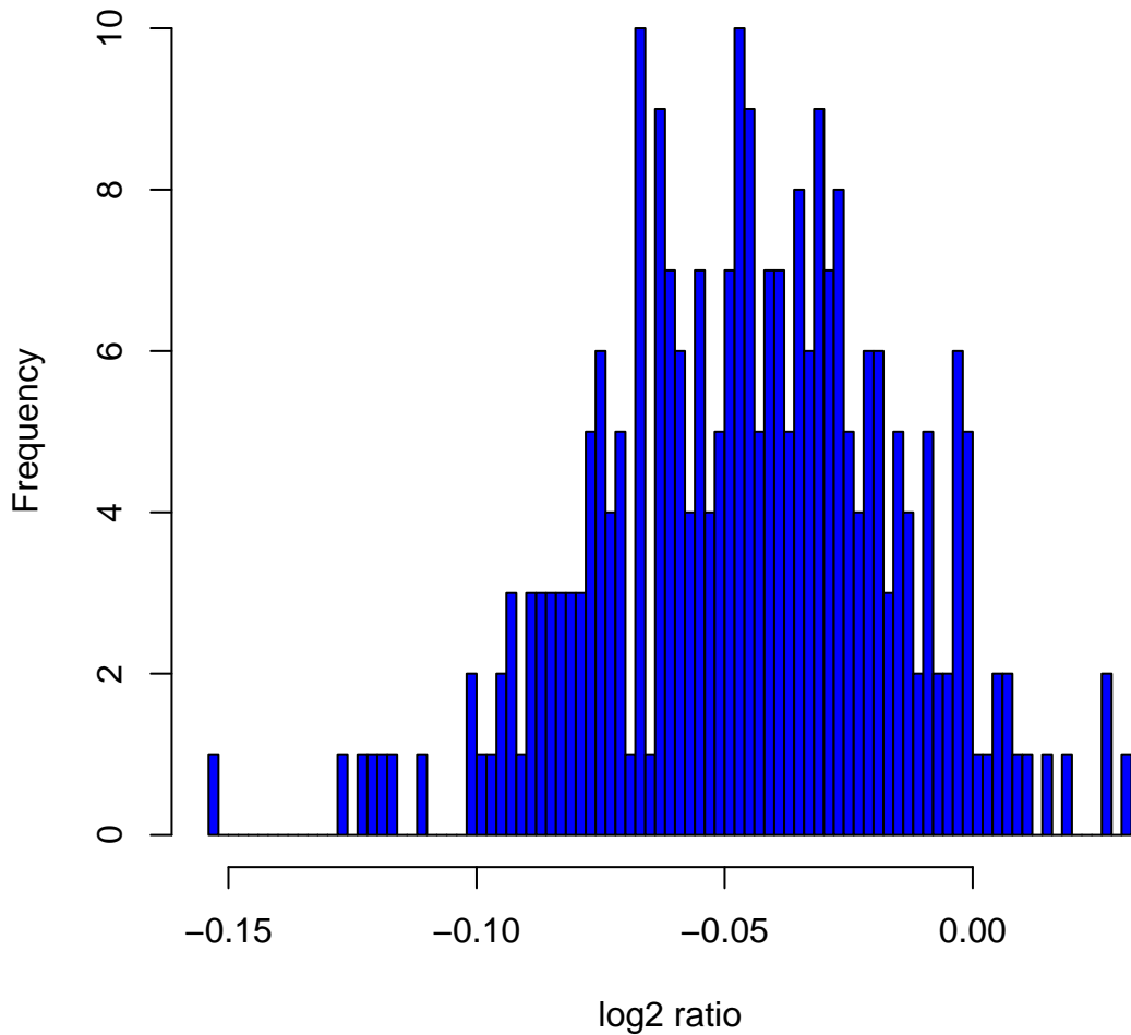
Histogram of log2ratios in 270 HapMap samples at clone Chr5tp-16H12
