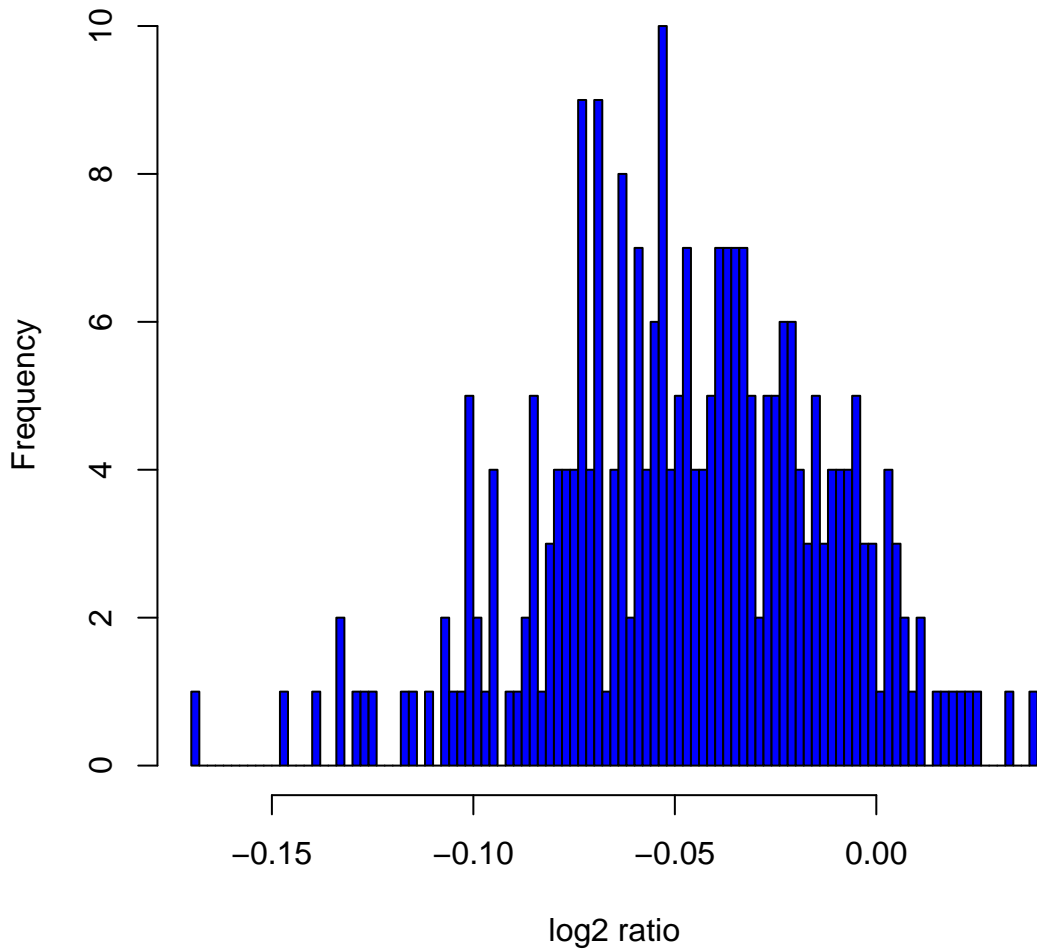
Histogram of log 2 ratios in 270 HapMap samples at clone Chr5tp-16H5
