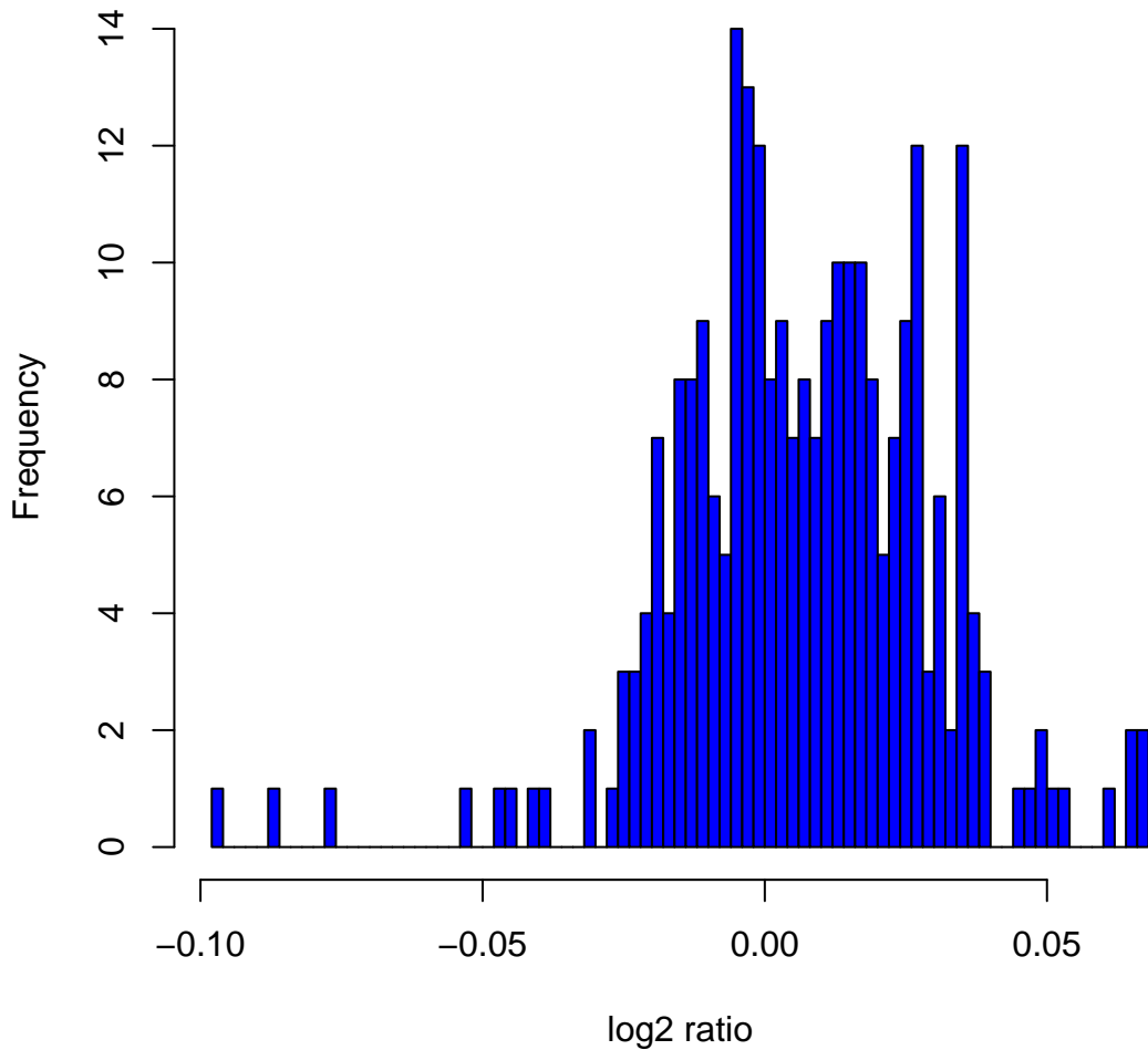
Histogram of log 2 ratios in 270 HapMap samples at clone Chr5tp-17C8
