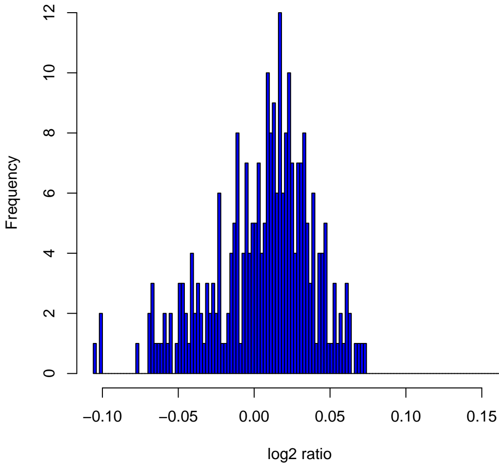
Histogram of log2ratios in 270 HapMap samples at clone Chr5tp-17E2
