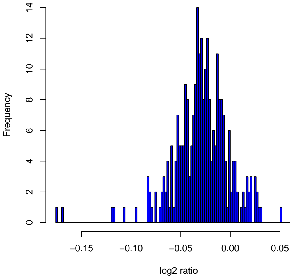
Histogram of log2ratios in 270 HapMap samples at clone Chr5tp-17E7
