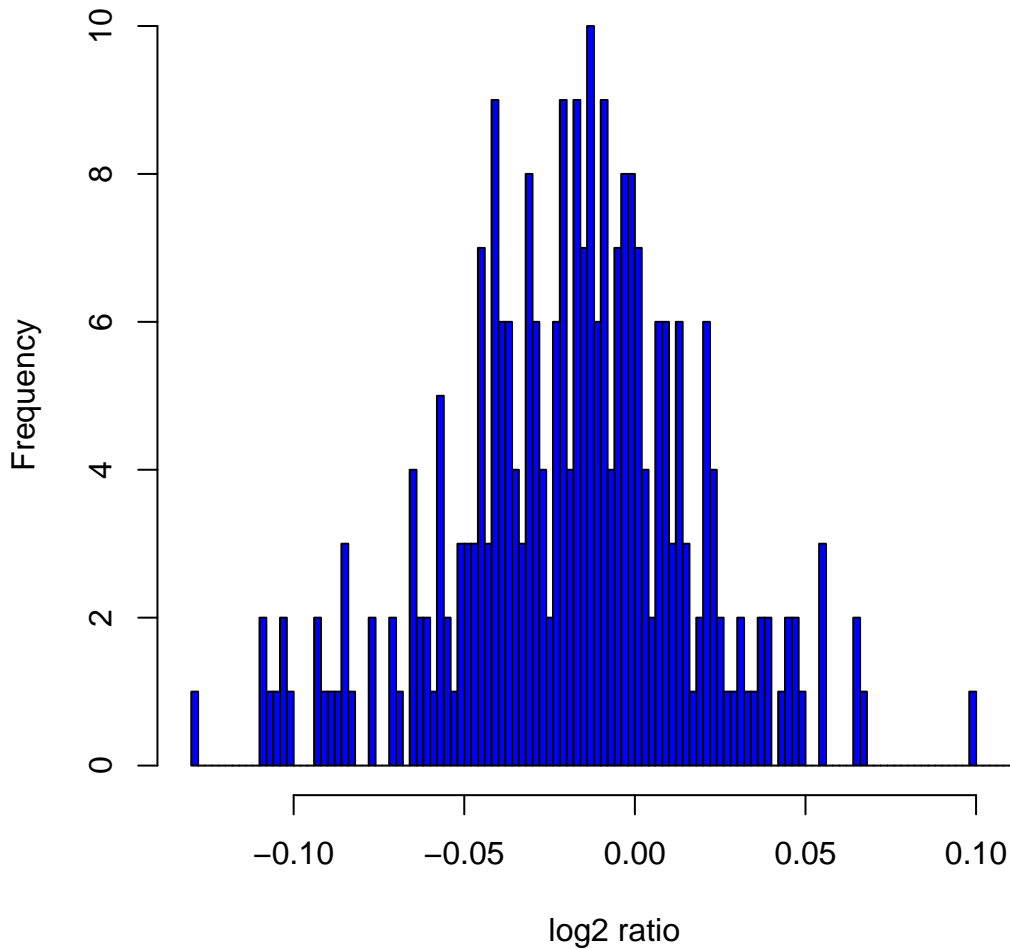
Histogram of \log_2 ratios in 270 HapMap samples at clone Chr5tp-17G4
