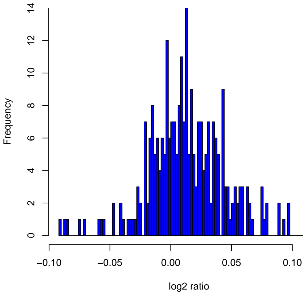
Histogram of log2ratios in 270 HapMap samples at clone Chr5tp-17H10
