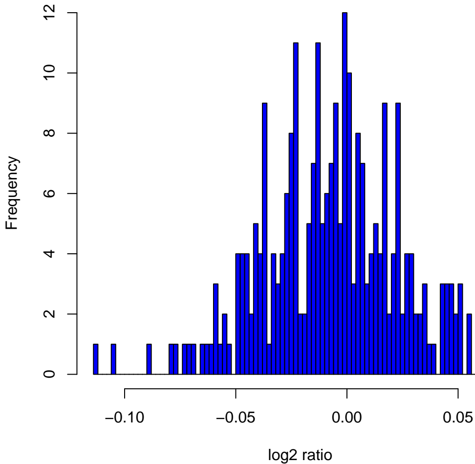
Histogram of \log_2 ratios in 270 HapMap samples at clone Chr5tp-18D4
