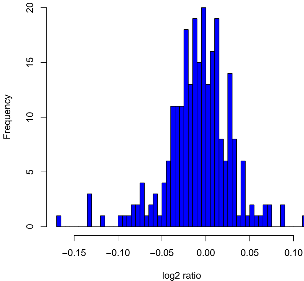
Histogram of log 2 ratios in 270 HapMap samples at clone Chr5tp-18F8
