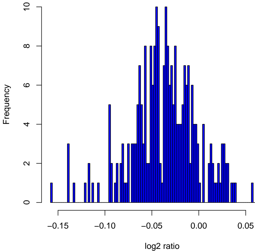
Histogram of log2ratios in 270 HapMap samples at clone Chr5tp-18H12
