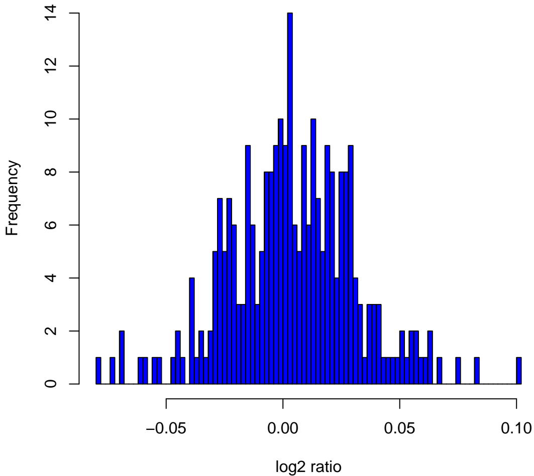
Histogram of log2ratios in 270 HapMap samples at clone Chr5tp-19A10
