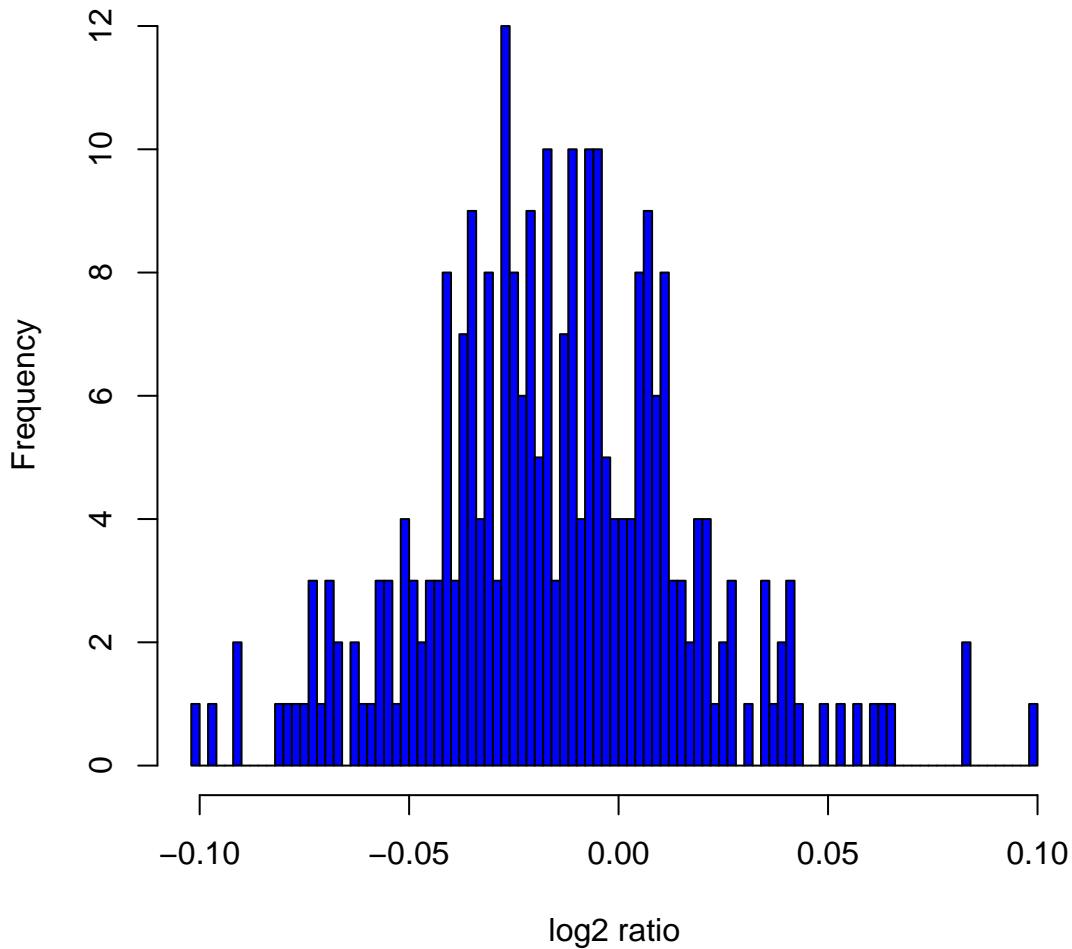
Histogram of \log_2 ratios in 270 HapMap samples at clone Chr5tp-19A3
