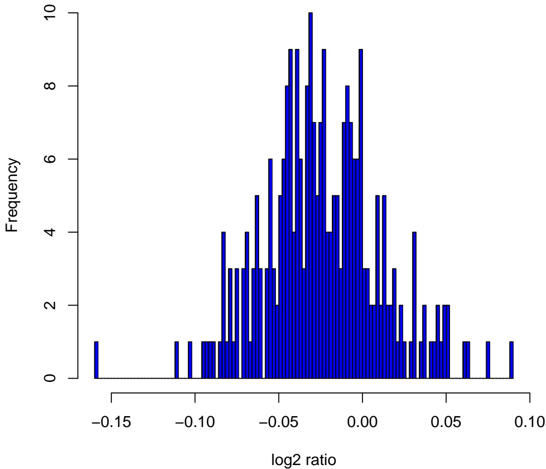
Histogram of \log_2 ratios in 270 HapMap samples at clone Chr5tp-19A7
