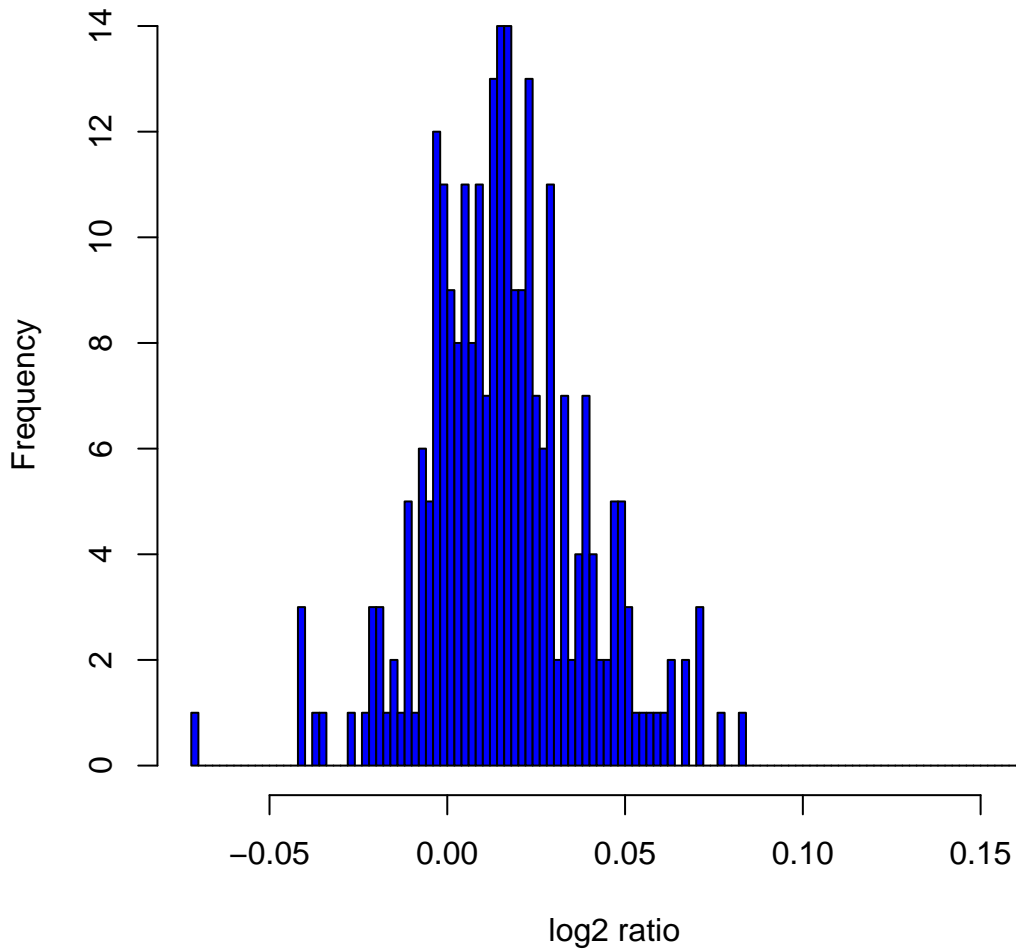
Histogram of log 2 ratios in 270 HapMap samples at clone Chr5tp-19E5
