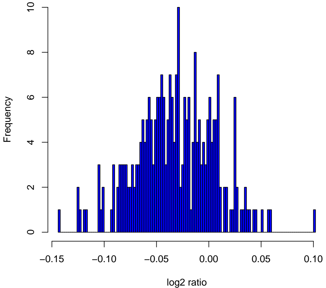
Histogram of log 2 ratios in 270 HapMap samples at clone Chr5tp-19H8
