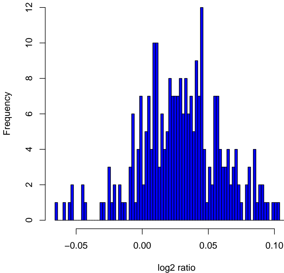
Histogram of log 2 ratios in 270 HapMap samples at clone Chr5tp-1B12
