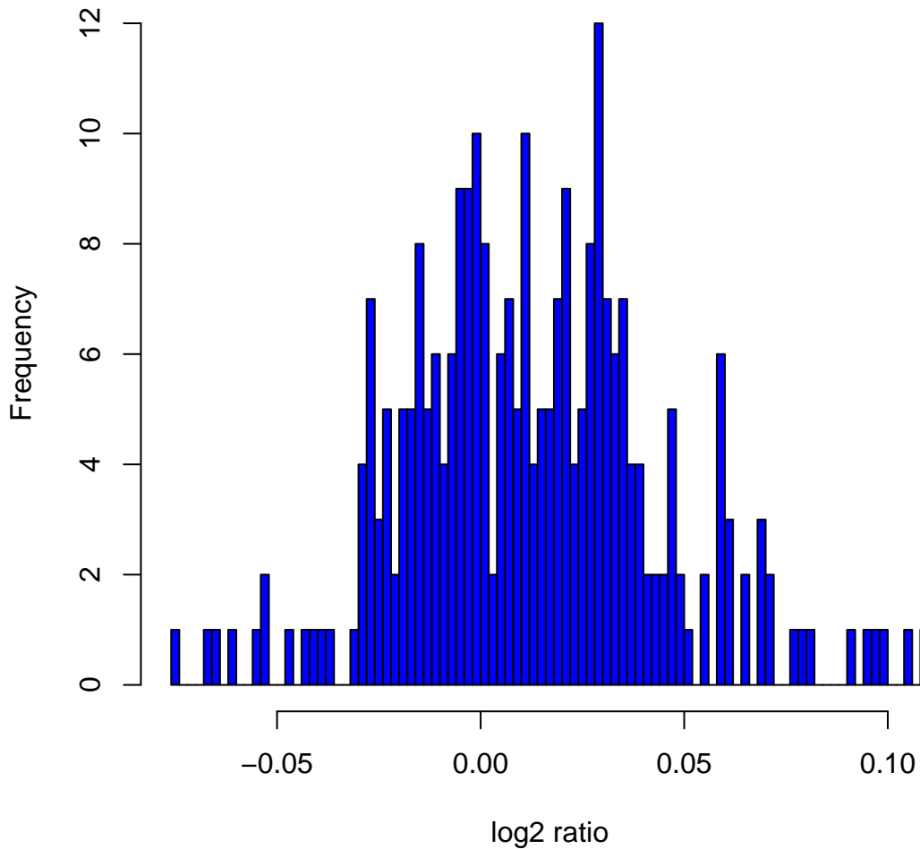
Histogram of log 2 ratios in 270 HapMap samples at clone Chr5tp-1B5
