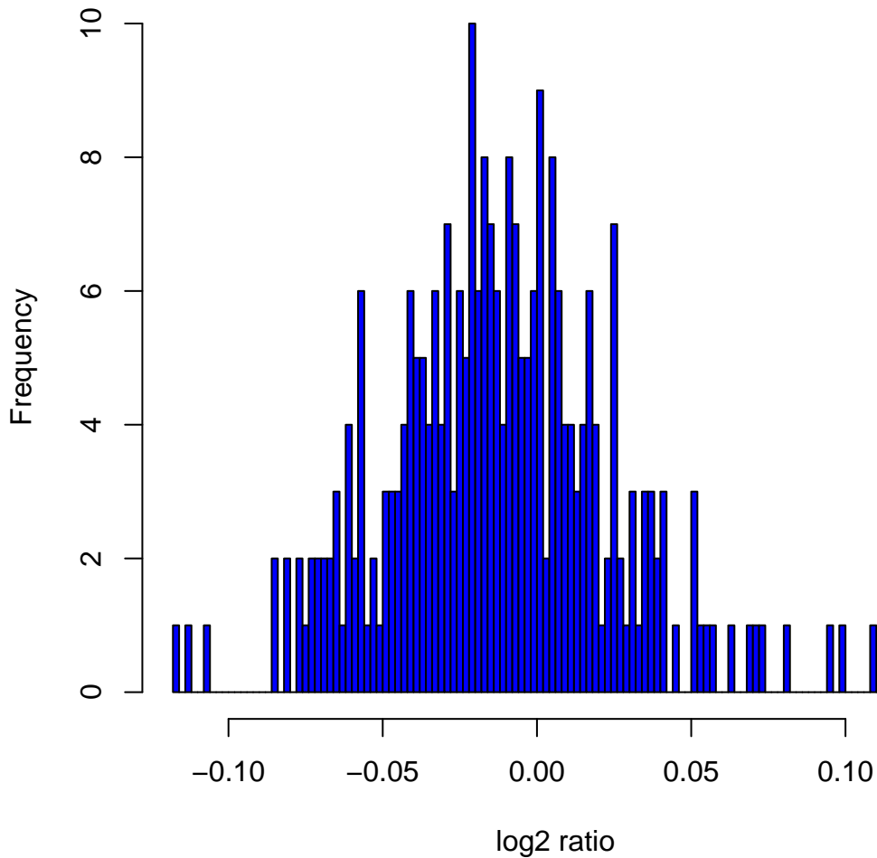
Histogram of \log_2 ratios in 270 HapMap samples at clone Chr5tp-1B7
