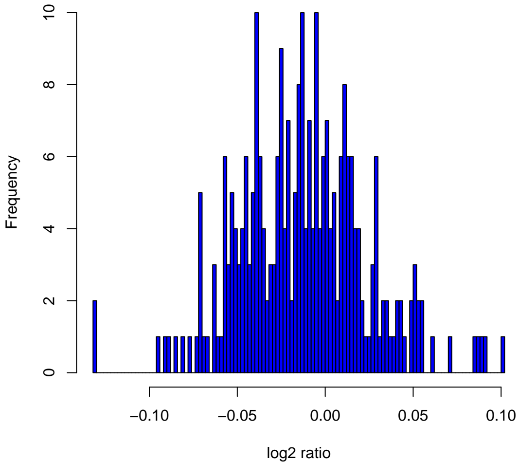
Histogram of \log_2 ratios in 270 HapMap samples at clone Chr5tp-1C11
