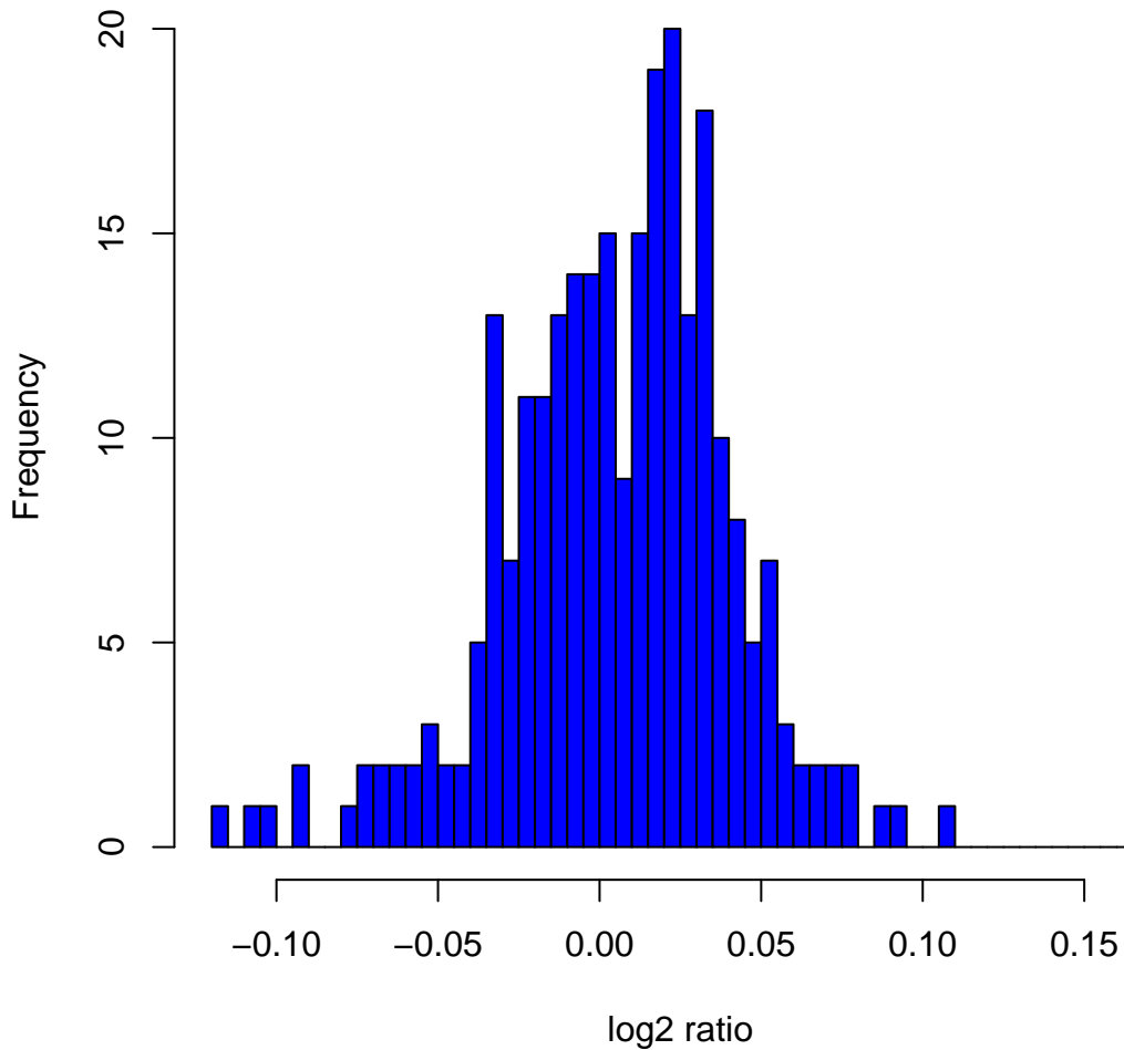
Histogram of log 2 ratios in 270 HapMap samples at clone Chr5tp-1C2
