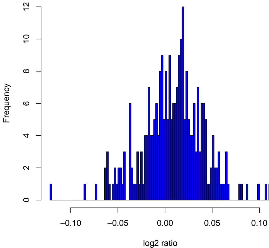
Histogram of log 2 ratios in 270 HapMap samples at clone Chr5tp-1C6
