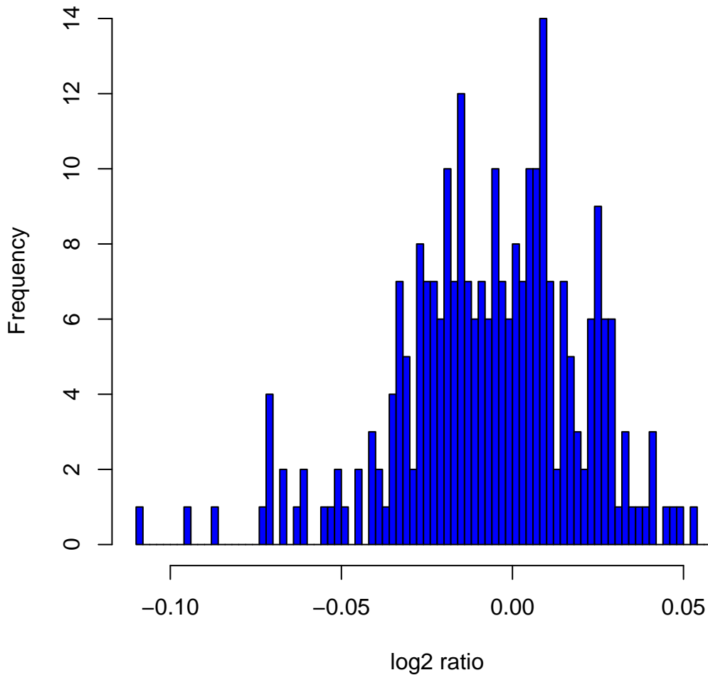
Histogram of \log_2 ratios in 270 HapMap samples at clone Chr5tp-1C8
