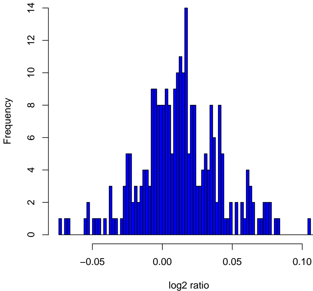
Histogram of log 2 ratios in 270 HapMap samples at clone Chr5tp-1D4
