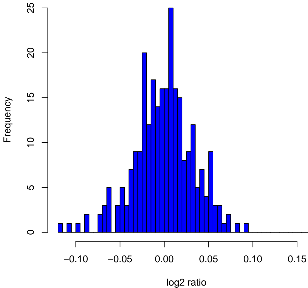
Histogram of log2ratios in 270 HapMap samples at clone Chr5tp-1E4
