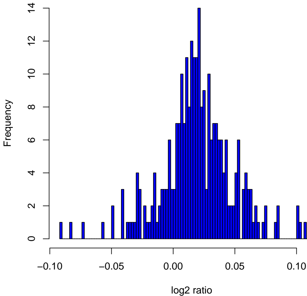
Histogram of log 2 ratios in 270 HapMap samples at clone Chr5tp-1G10
