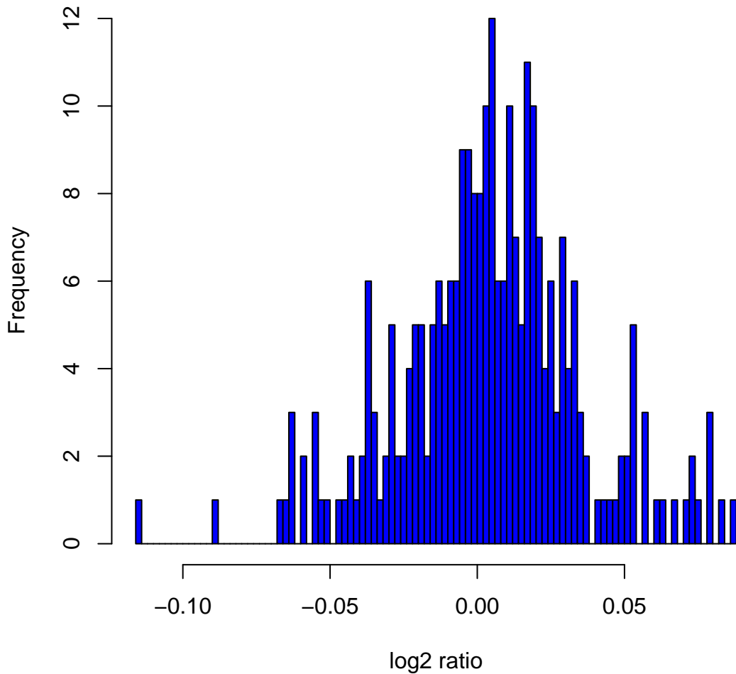
Histogram of log 2 ratios in 270 HapMap samples at clone Chr5tp-1H6
